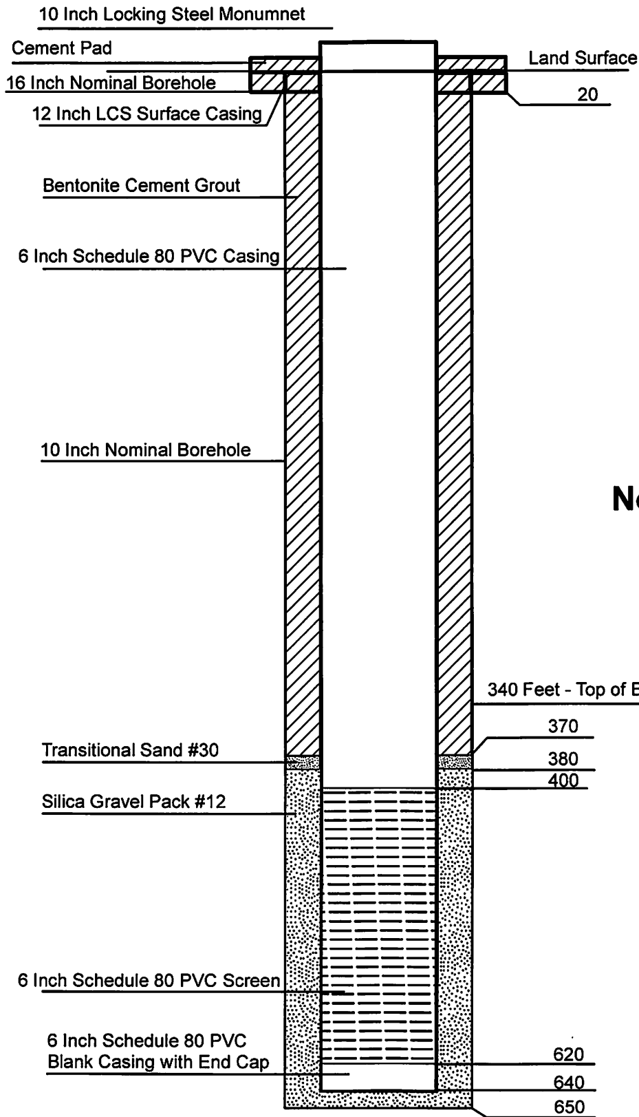
PW2-1 Well Diagram
